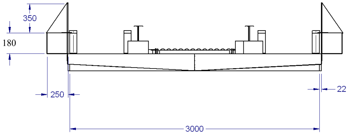
Face view
